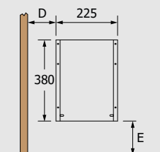
Wall Mounting Rack Installation
