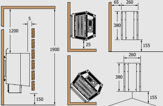
Wall Mounting Rack Installation
