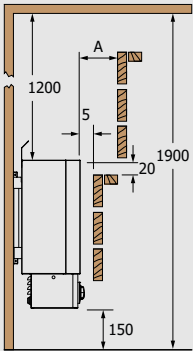
Wall Mounting Rack Installation
