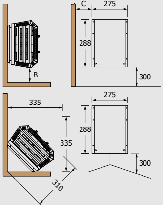
Wall Mounting Rack Installation
