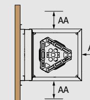
Wall Installation with Protective Cover
