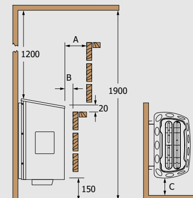
Wall Mounting Rack Installation
