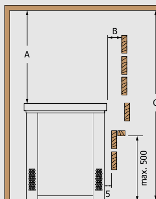
Minimum Safety Distances
