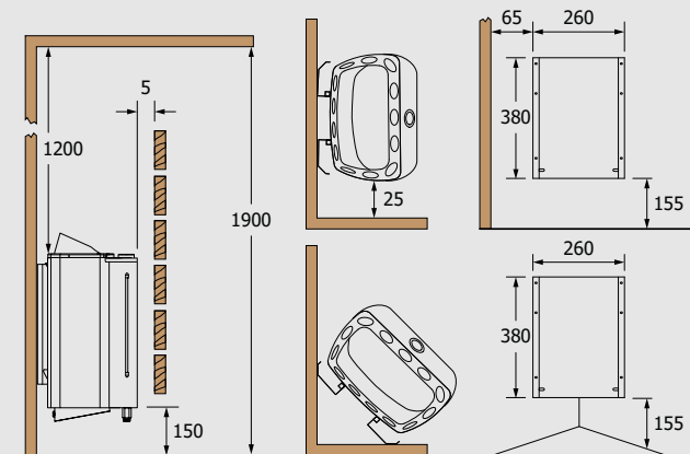
Wall Mounting Rack Installation
